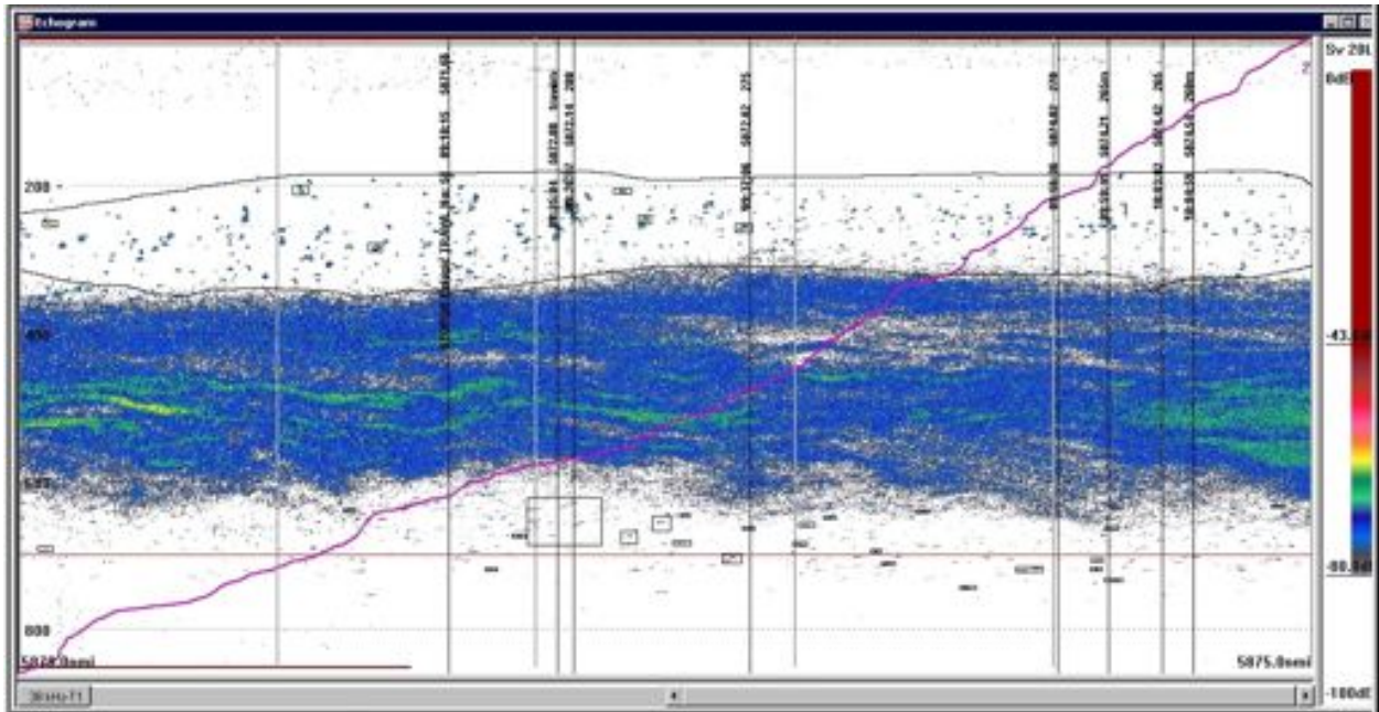
Figure 12.1. Echogram recorded by Russian RV “Smolensk” over 5 nautical miles during the summer 2007 survey in the Irminger Sea (38KHz, pulse length 2 ms). The dense layer is the deep scattering layer (DSL) in which redfish are mixed with other small organisms. Pure redfish aggregations distinctly visible above DSL in the acoustic layer (contoured by layer tool of scrutinizing software). Single targets of redfish below DSL are also visible (contoured by rectangles). Reproduced from ICES (2007).
