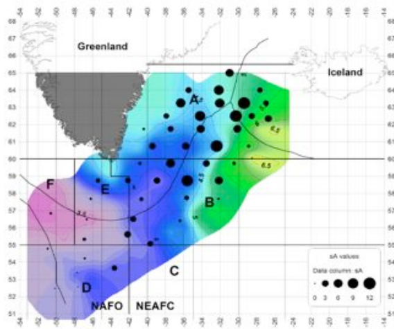
Figure 14.1. Temperature distribution (colour) and redfish distribution (bubbles) as recorded during the international redfish survey in the Irminger Sea and adjacent waters in June/July 2009. Top-left: temperature at 200m depth and redfish distribution derived from hydroacoustics. Top-right: temperature at 400m depth and trawl-catches shallower than 500m. Bottom-left: temperature at 600m depth and trawl-catches deeper than 500m.
